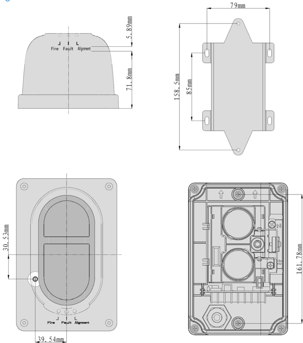
Figure 2: Detector Diagram
