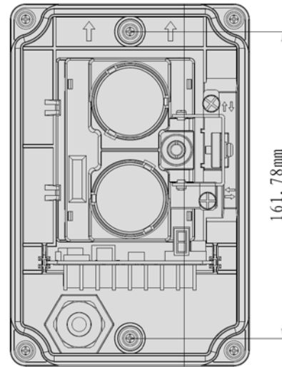
Figure 5: Beam Detector
